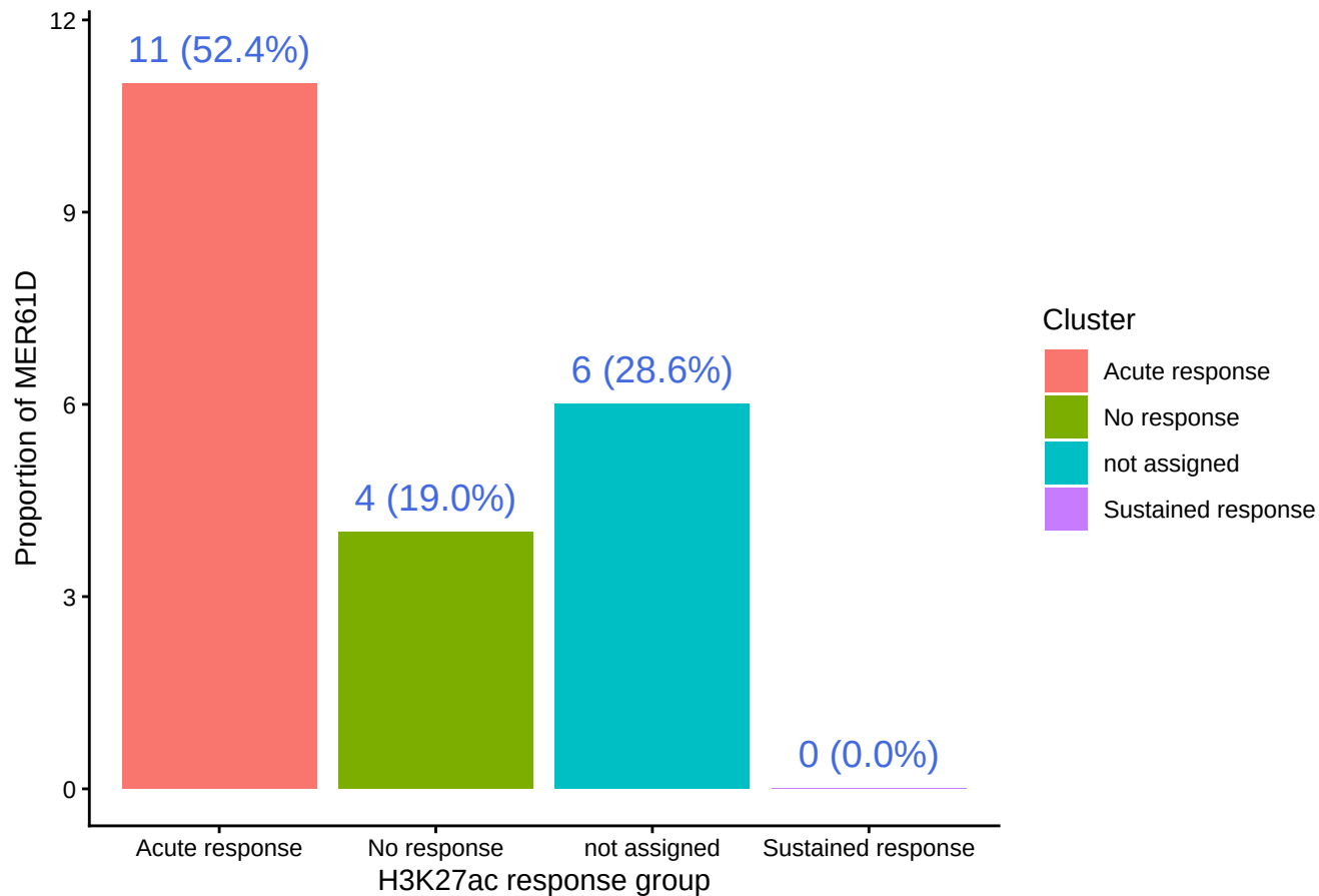
Proportion of MER61D across each H3K27ac set
